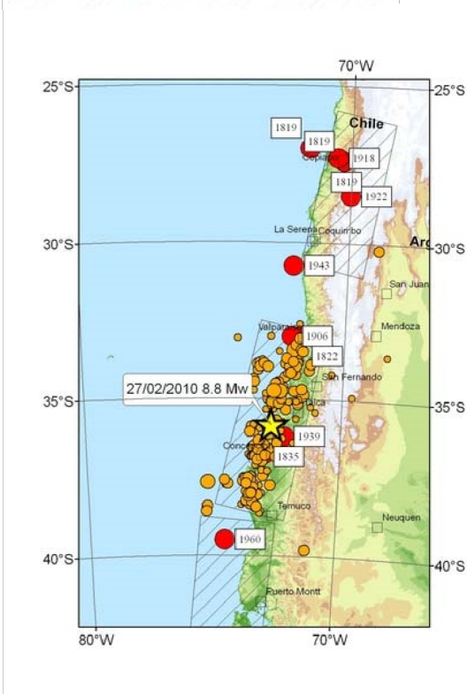
Figure 8. Aftershocks of Chile great earthquake compared to epicentre (large dot) which lies toward the base of rupture.
