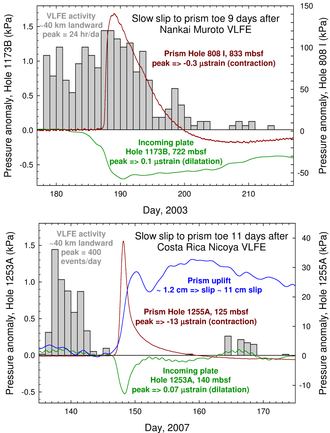
Figure 4. Formation and seafloor pressures recorded at ODP borehole sites seaward and landward of the frontal thrusts of the Nankai and Costa Rica subduction zones. These detailed records illustrate deformation associated with slow slip that begins several tens of km landward (as defined by very low frequency earthquake activity), and propagates to the prism toe over the course of several days. At Costa Rica, the reduction in pressure associated with dilatation is not maintained because of high crustal permeability and a short hydrologic drainage path.
